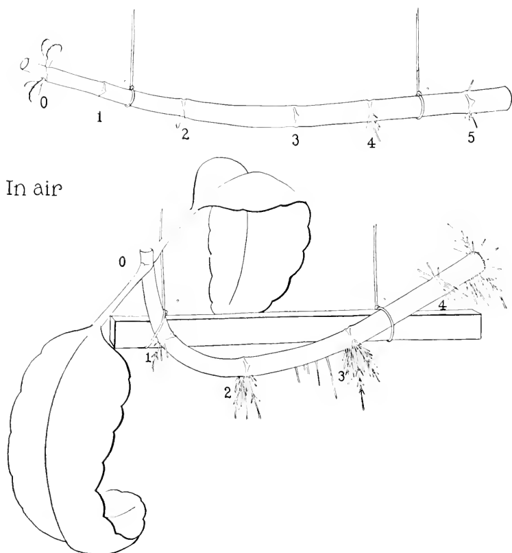
FIG. 64.—Roots grow on under side of stems suspended horizontally, but more roots grow when there is a leaf at the apex of the stem. Nov. 18 to Dec. 13, 1923.
